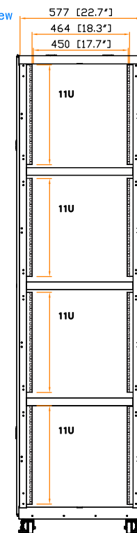
19" rail position
