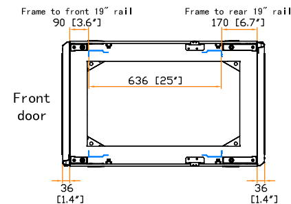
19" rail position
