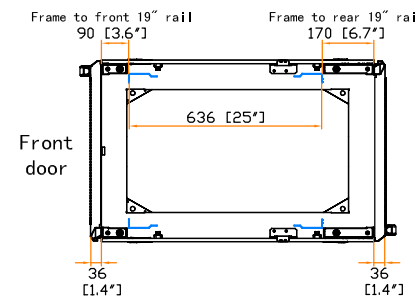
19" rail position
