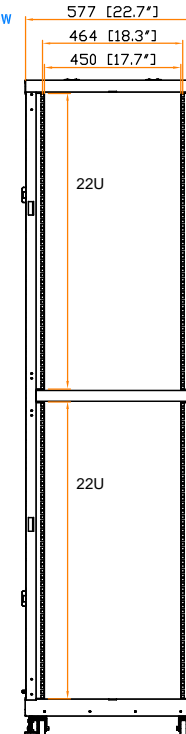
19" rail position
