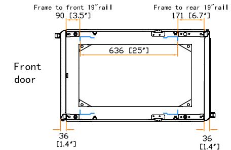
19" rail position
