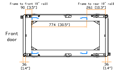
19" rail position
