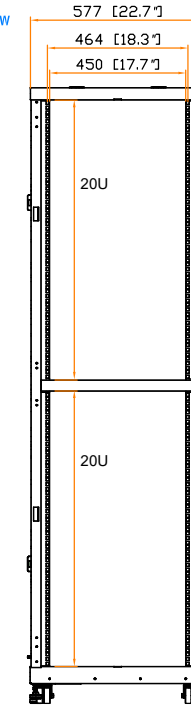
19" rail position
