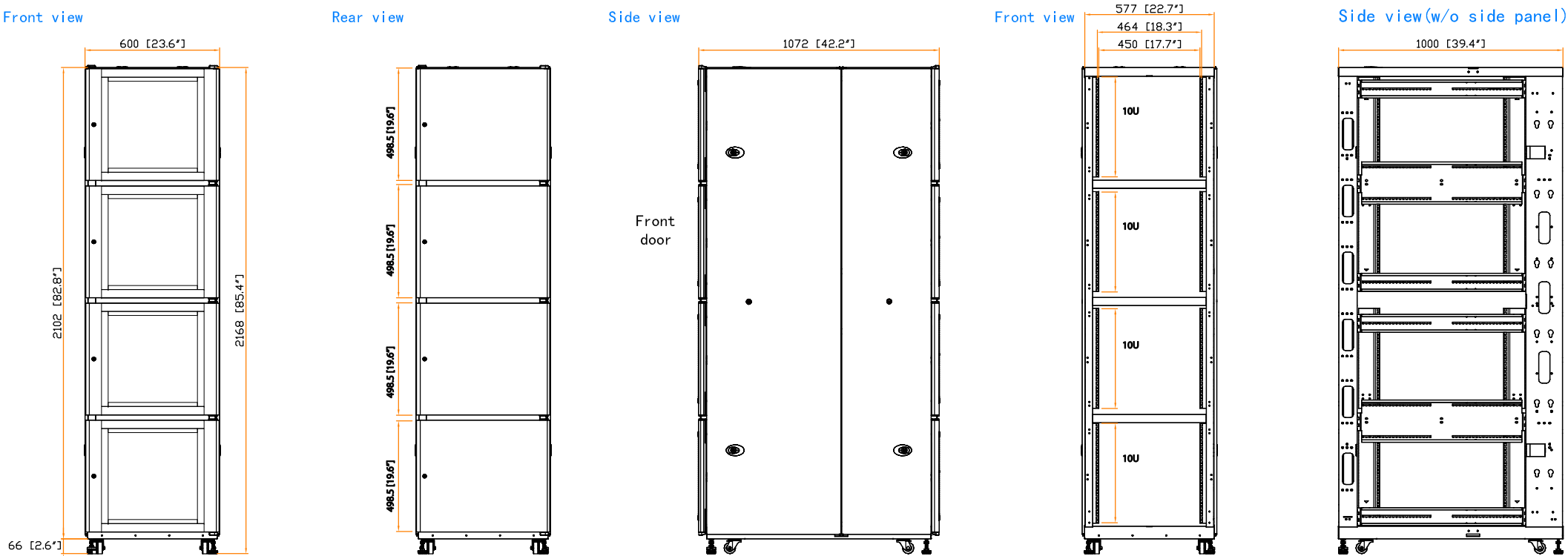
19" rail position
